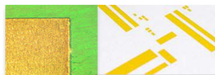
Solder mask removal (L) and coverlay kiss-cuts (R).
