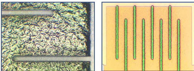
Serpentine legs in thin film on Si with 10 \mu\text{m} kerf (R) and thick film on alumina (L).
