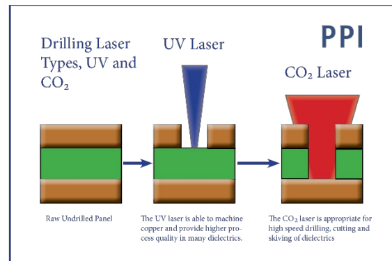
Figure 1: Drilling Laser Types
